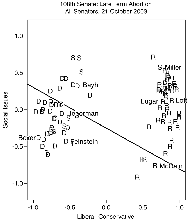
Fig. 1. Ideal points and cutting line for 21 October 2003 vote
